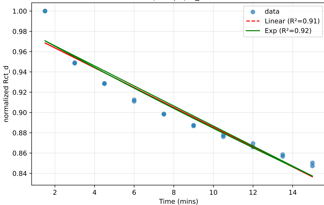
Chip 41 | 0pM_asso
